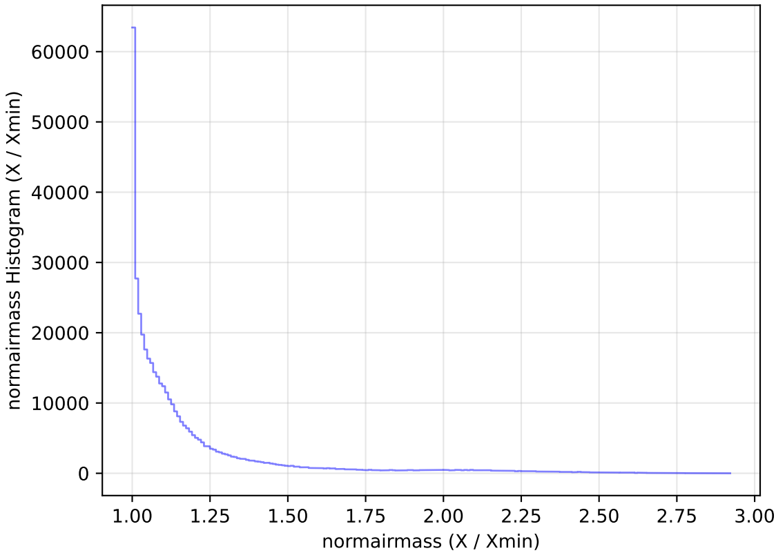
too_5_1v3.4_10yrs All sky z band: normairmass Histogram
