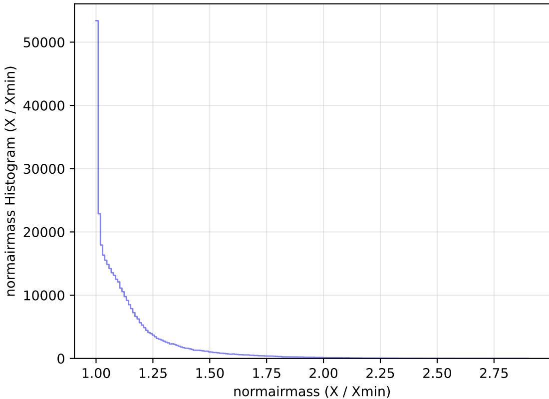
too_5_1v3.4_10yrs All sky y band: normairmass Histogram
