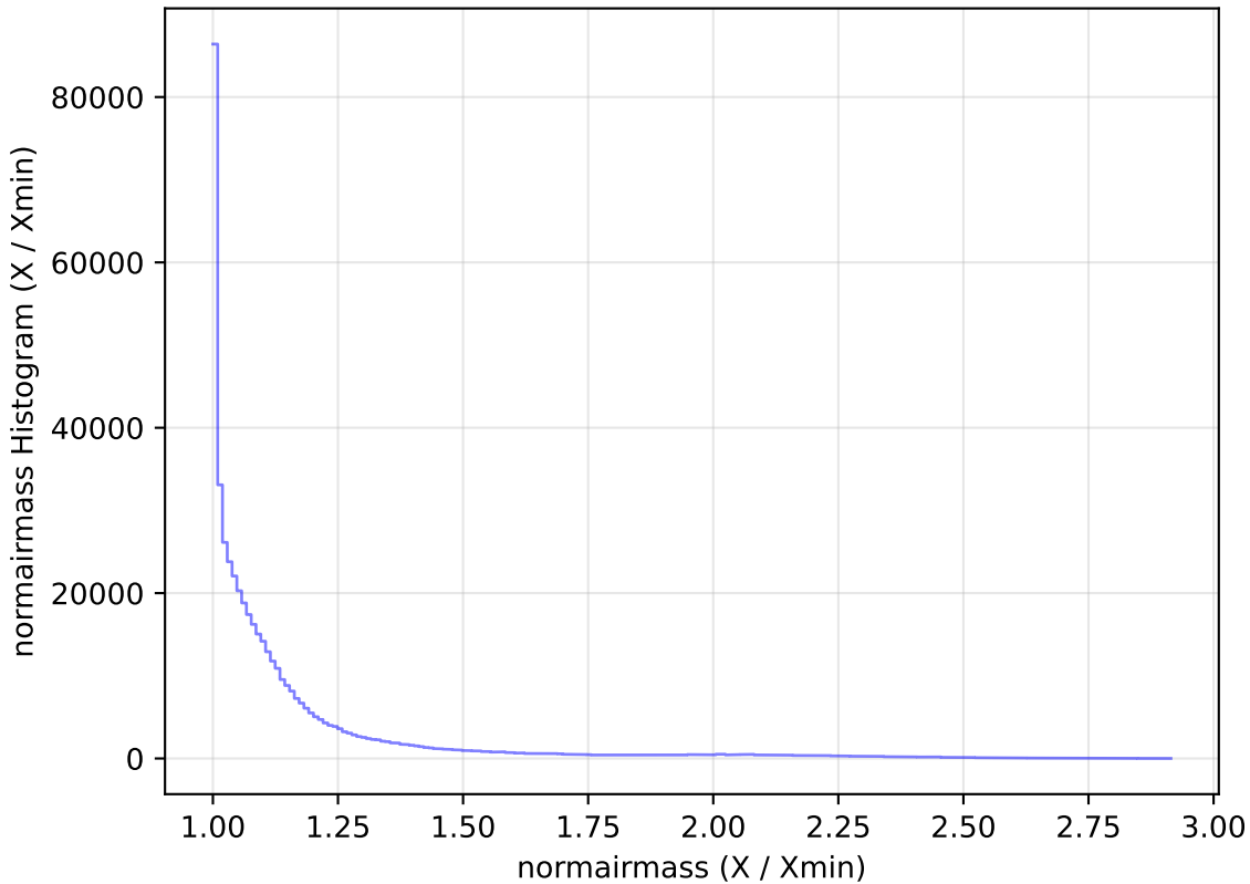
too_5_1v3.4_10yrs All sky i band: normairmass Histogram
