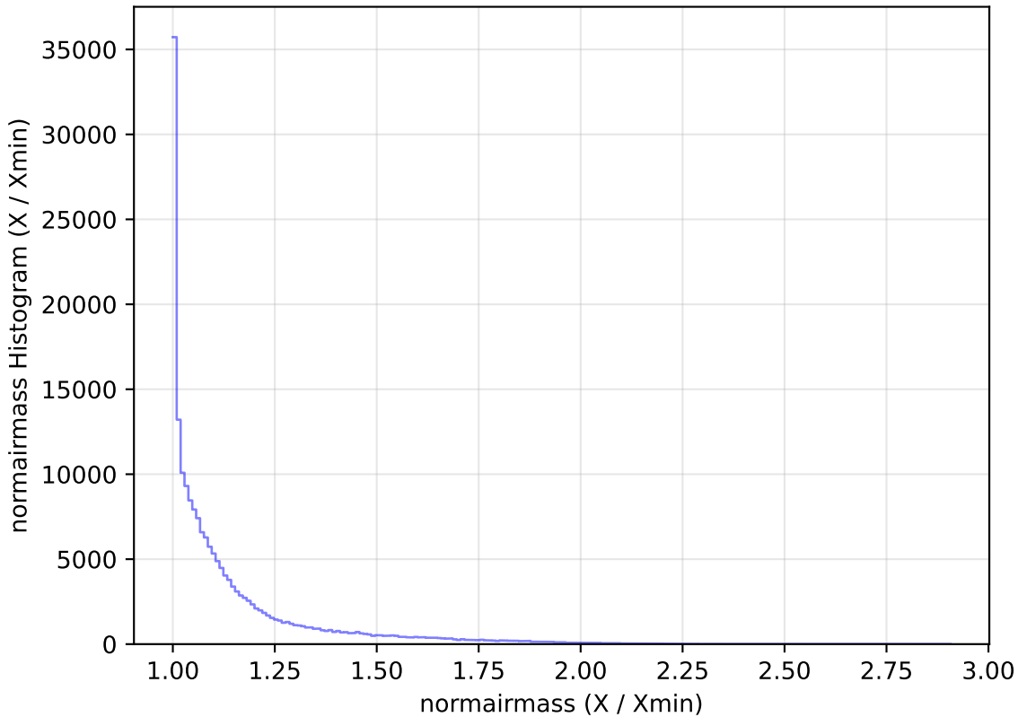
too_5_1v3.4_10yrs All sky g band: normairmass Histogram
