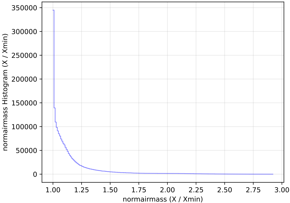
too_5_1v3.4_10yrs All sky all bands: normairmass Histogram
