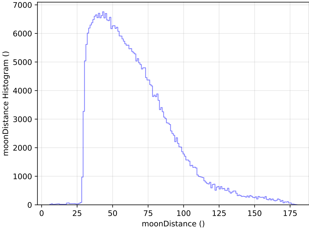
too_5_1v3.4_10yrs WFD y band: moonDistance Histogram
