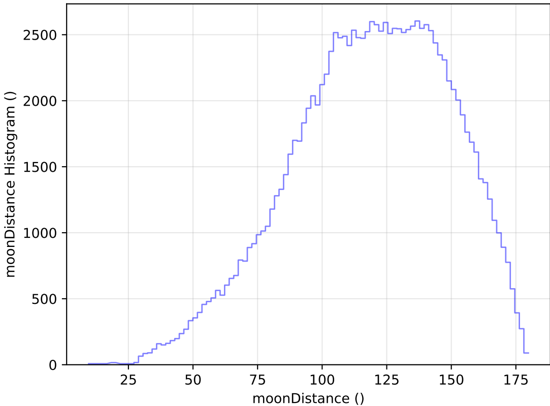
too_5_1v3.4_10yrs WFD u band: moonDistance Histogram
