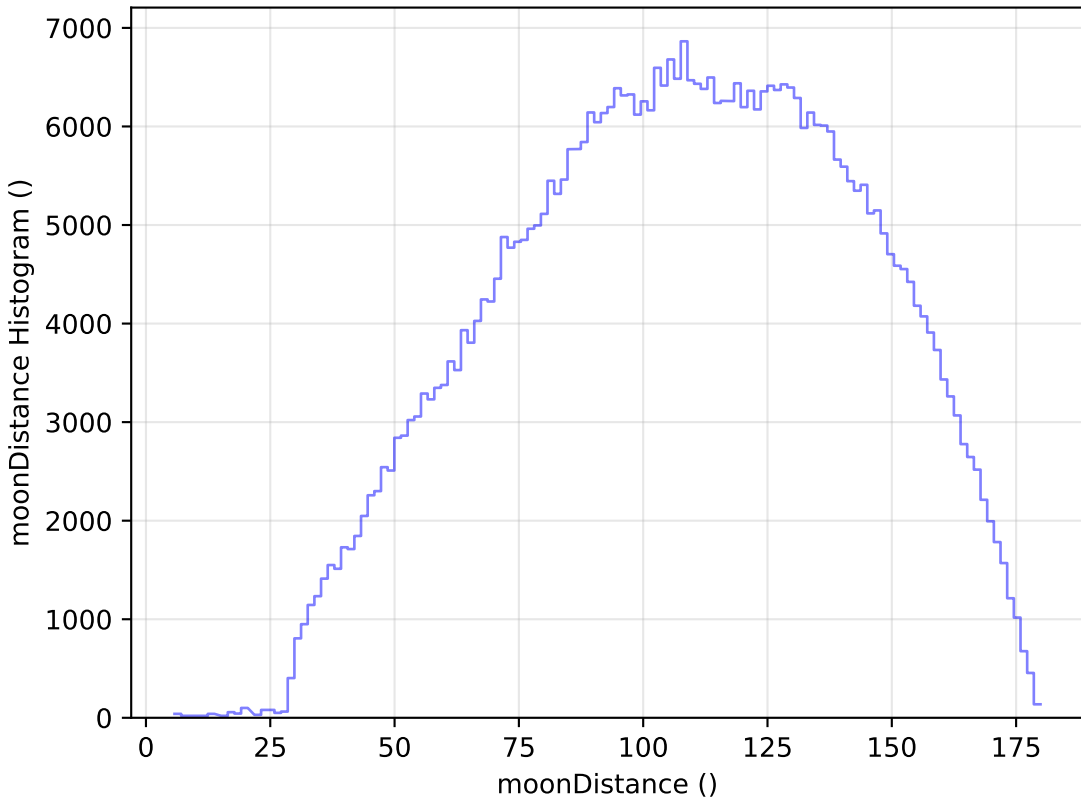
too_5_1v3.4_10yrs WFD r band: moonDistance Histogram
