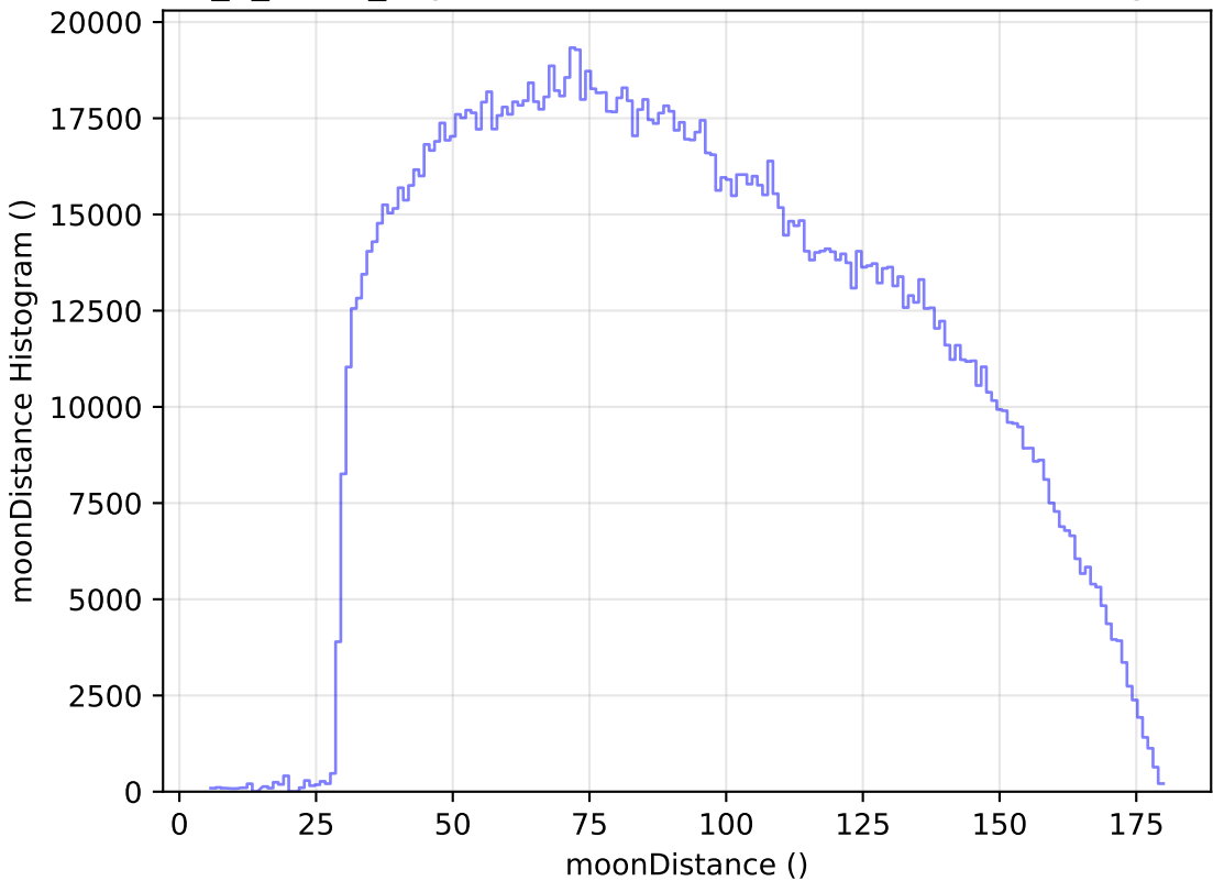
too_5_1v3.4_10yrs WFD all bands: moonDistance Histogram
