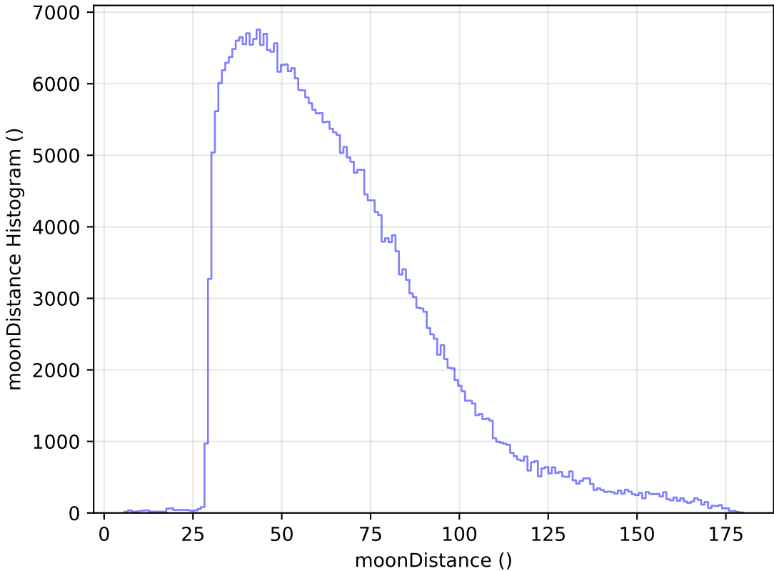
too_5_1v3.4_10yrs All sky y band: moonDistance Histogram
