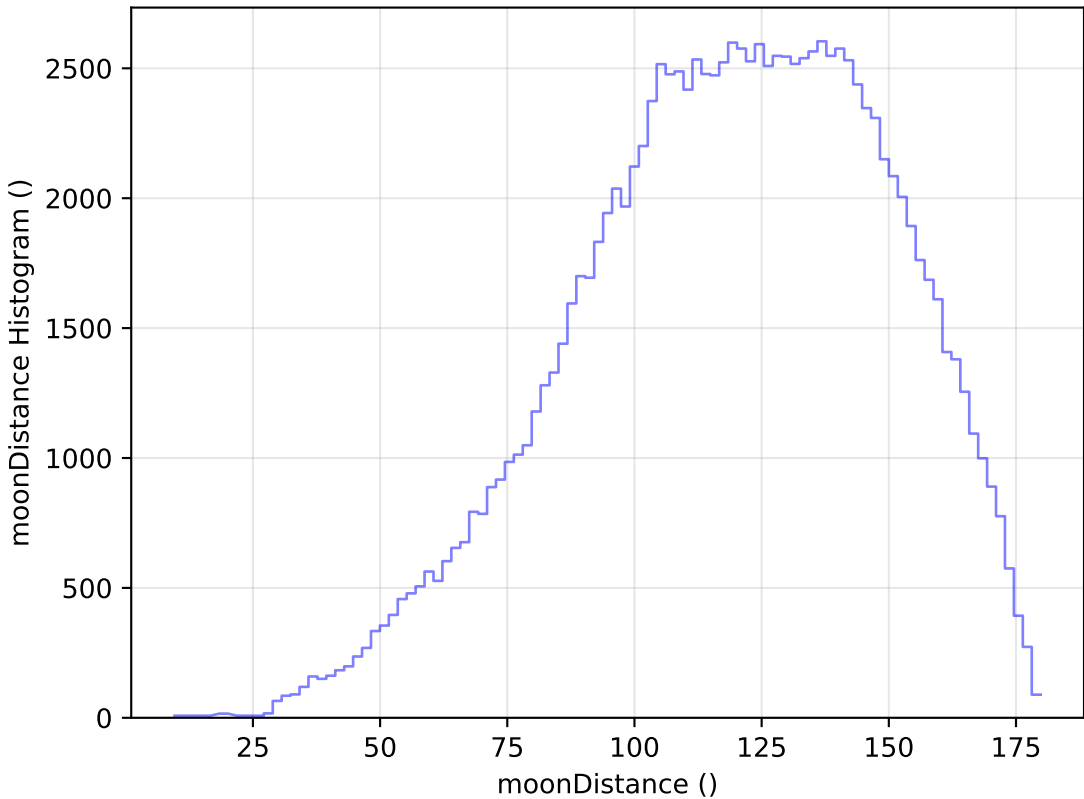
too_5_1v3.4_10yrs All sky u band: moonDistance Histogram
