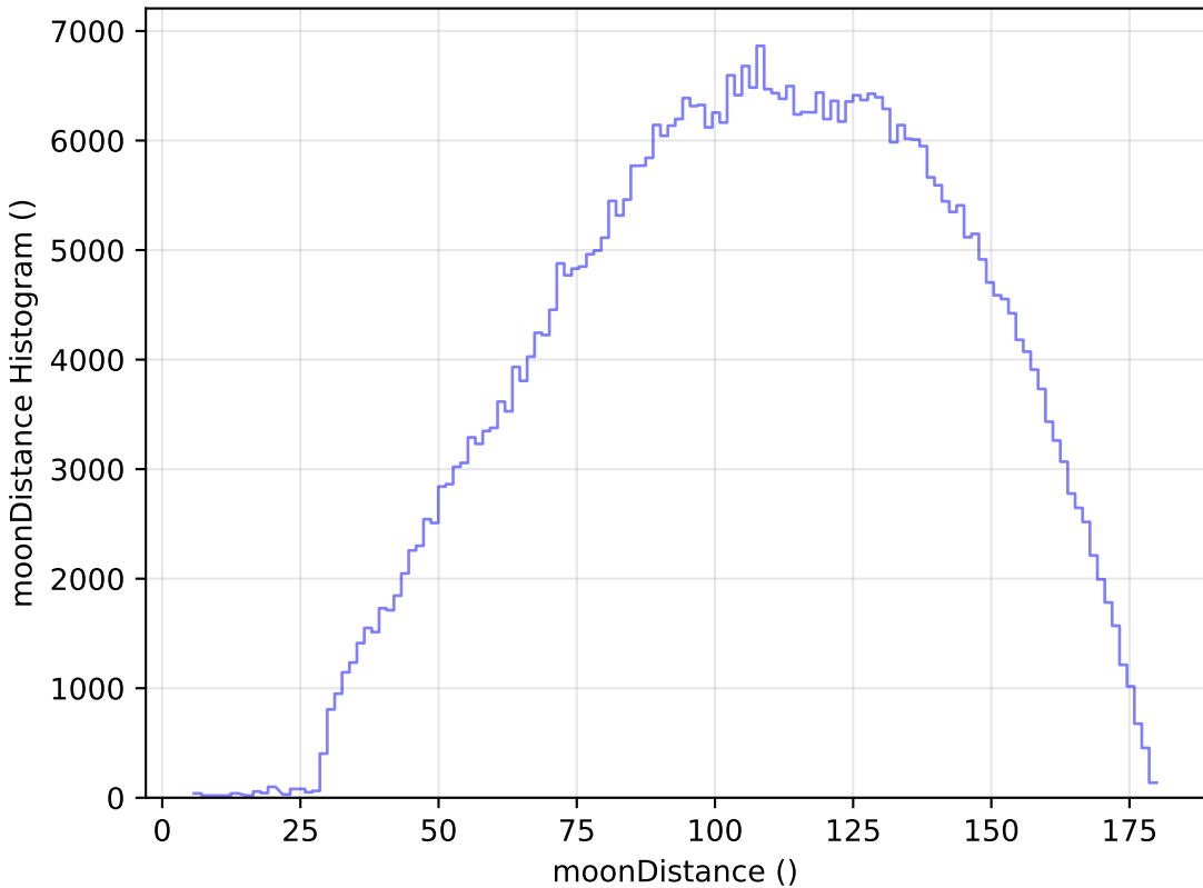
too_5_1v3.4_10yrs All sky r band: moonDistance Histogram
