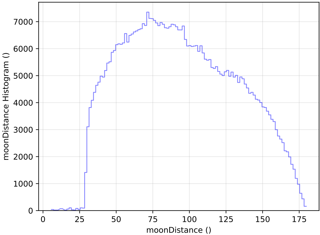
too_5_1v3.4_10yrs All sky i band: moonDistance Histogram
