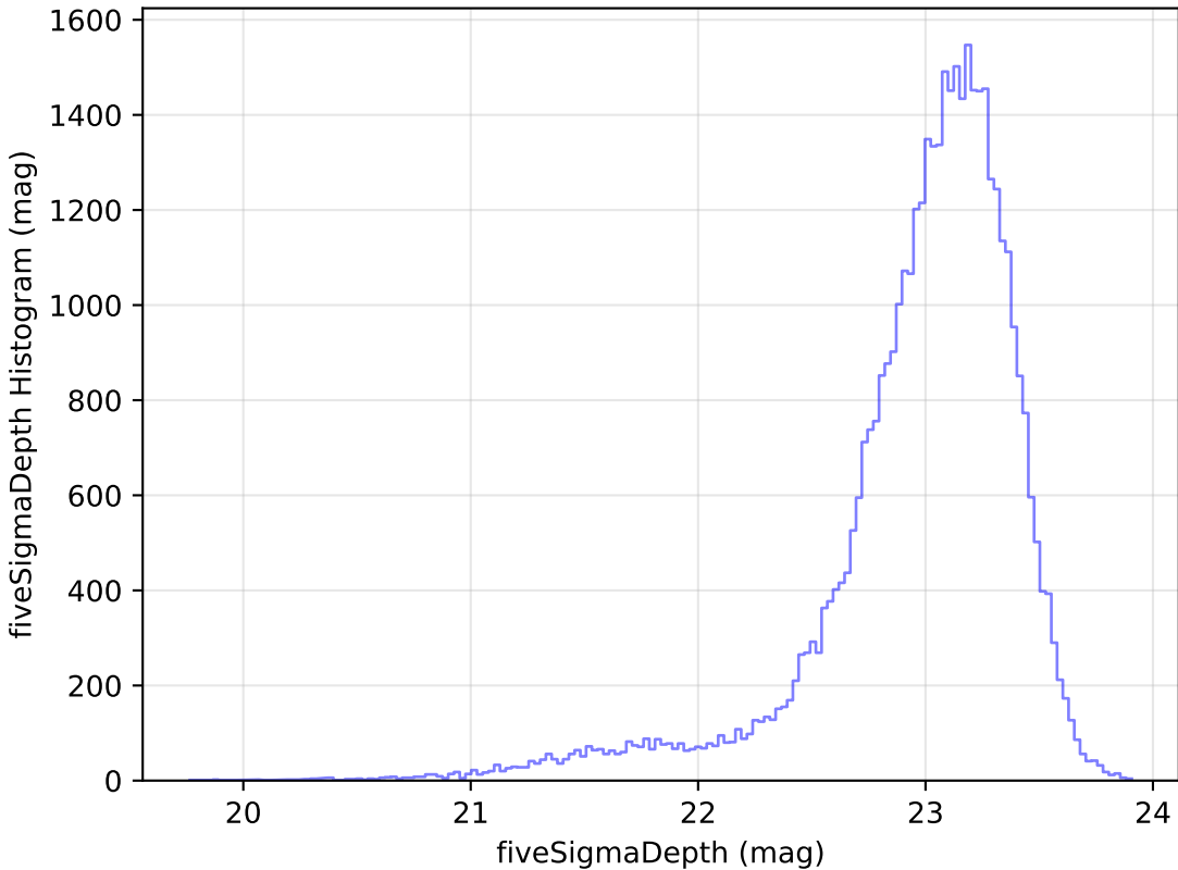
too_5_1v3.4_10yrs Yr 1 z band: fiveSigmaDepth Histogram
