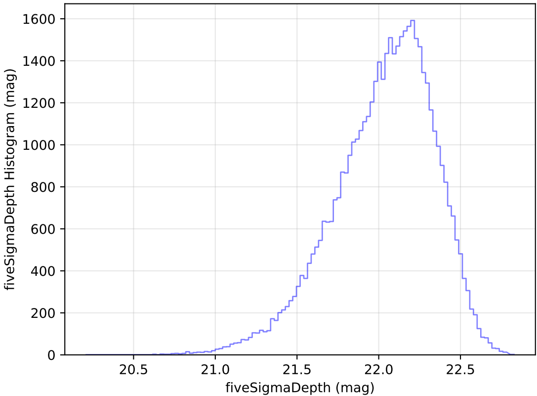
too_5_1v3.4_10yrs Yr 1 y band: fiveSigmaDepth Histogram
