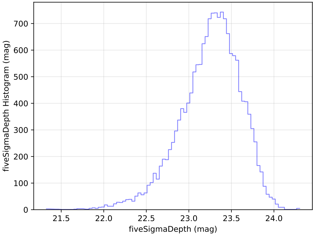
too_5_1v3.4_10yrs Yr 1 u band: fiveSigmaDepth Histogram
