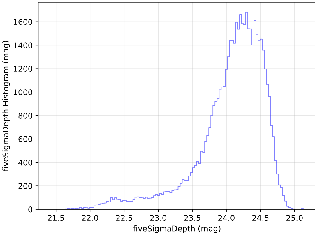
too_5_1v3.4_10yrs Yr 1 r band: fiveSigmaDepth Histogram
