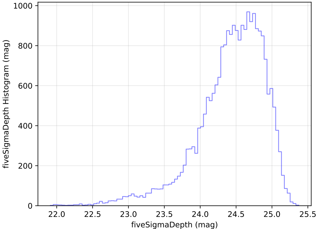
too_5_1v3.4_10yrs Yr 1 g band: fiveSigmaDepth Histogram
