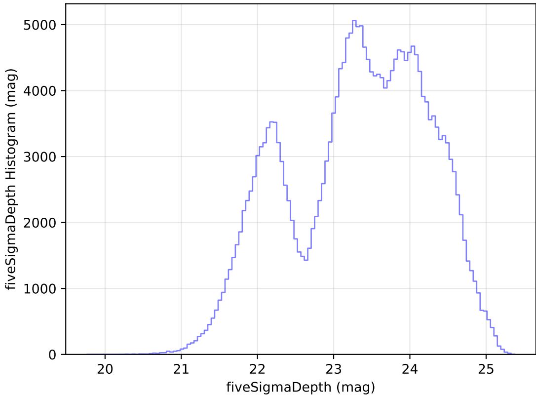
too_5_1v3.4_10yrs Yr 1 all bands: fiveSigmaDepth Histogram
