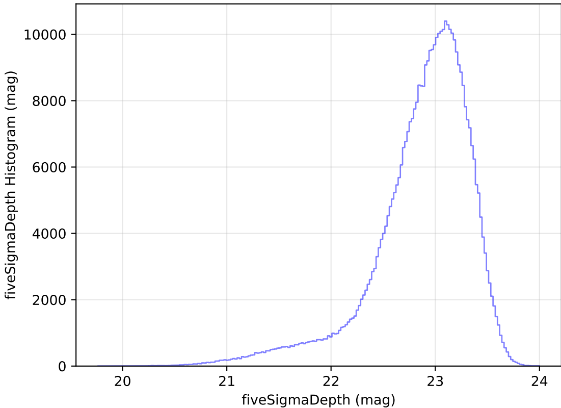
too_5_1v3.4_10yrs WFD z band: fiveSigmaDepth Histogram
