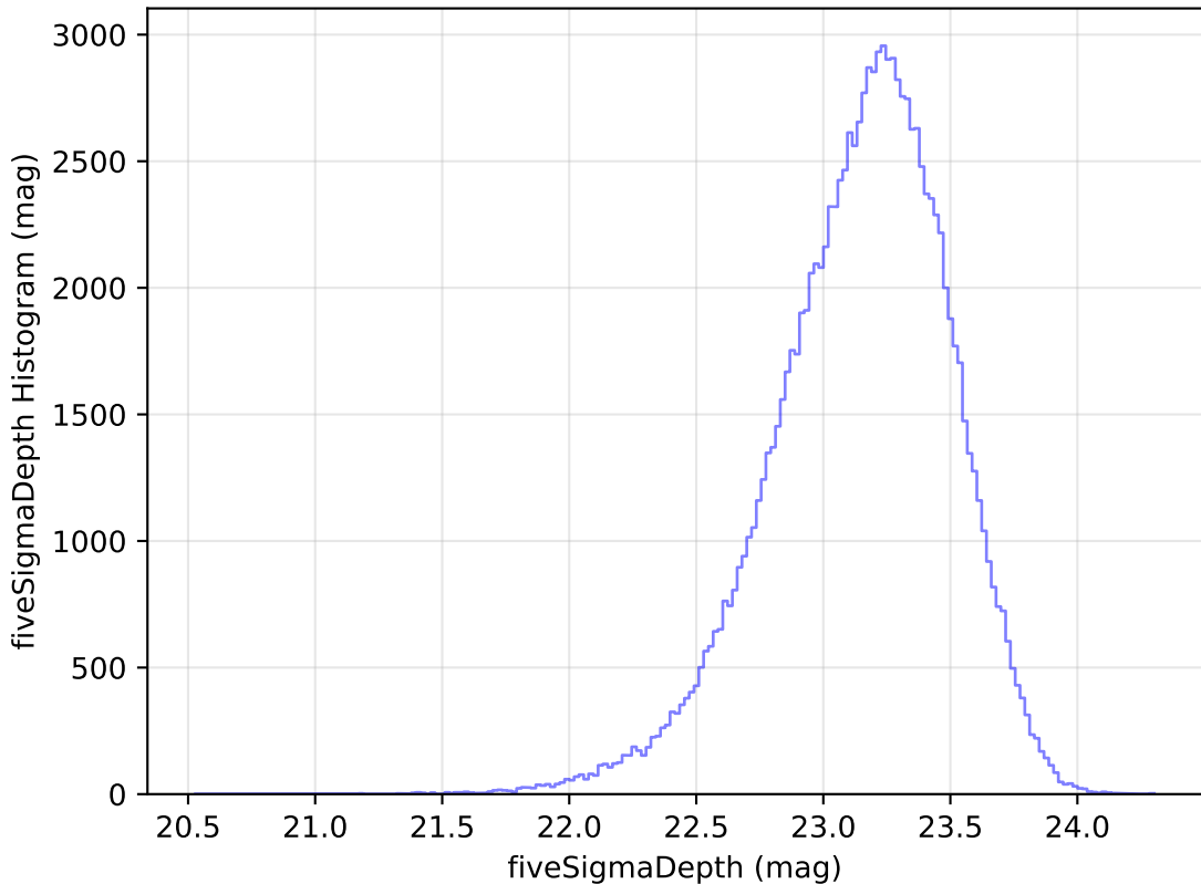
too_5_1v3.4_10yrs WFD u band: fiveSigmaDepth Histogram
