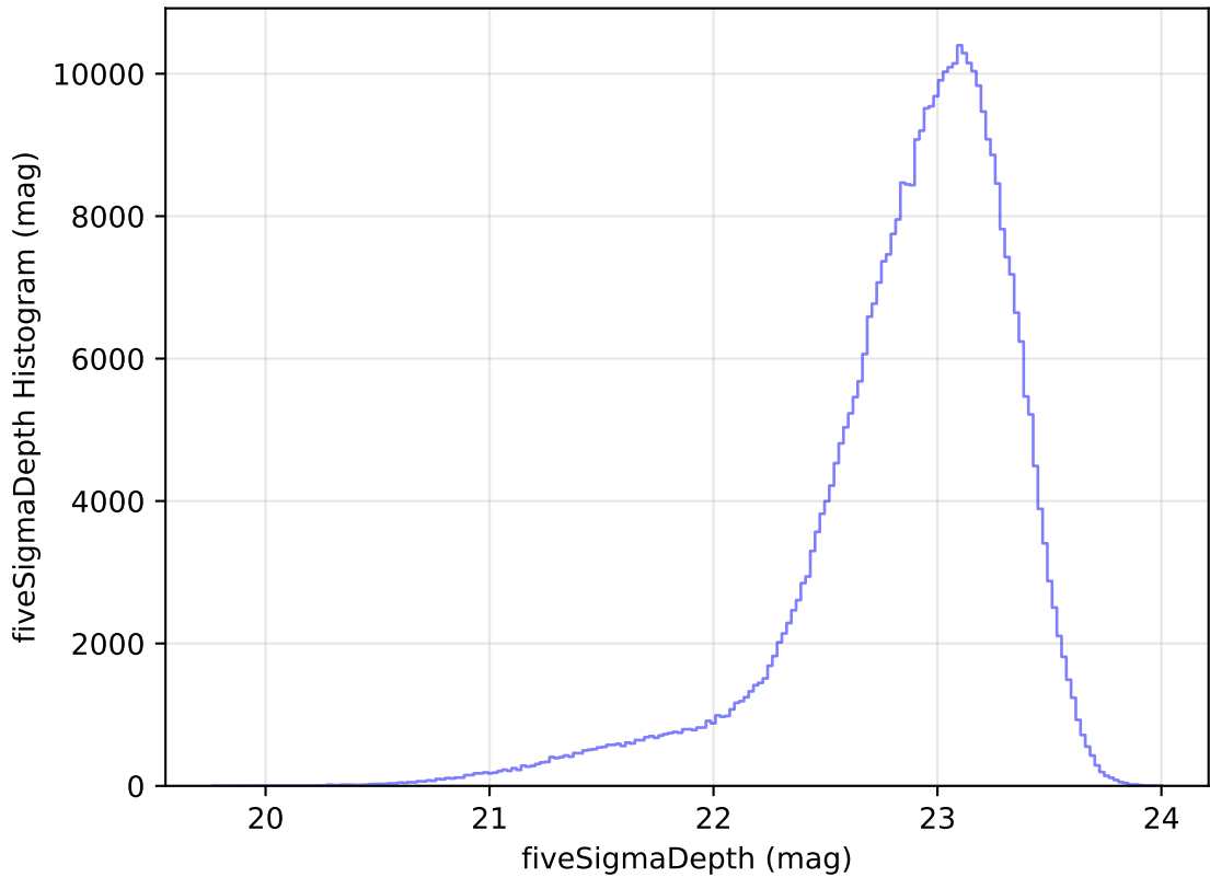
too_5_1v3.4_10yrs All sky z band: fiveSigmaDepth Histogram
