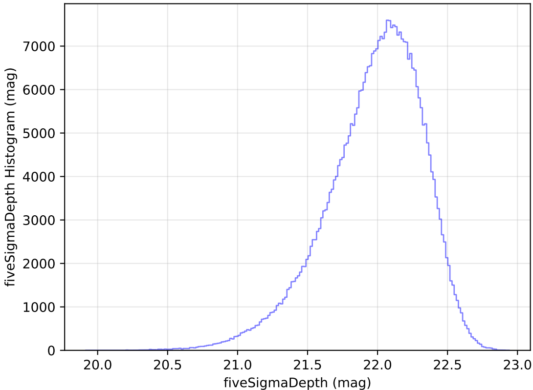
too_5_1v3.4_10yrs All sky y band: fiveSigmaDepth Histogram
