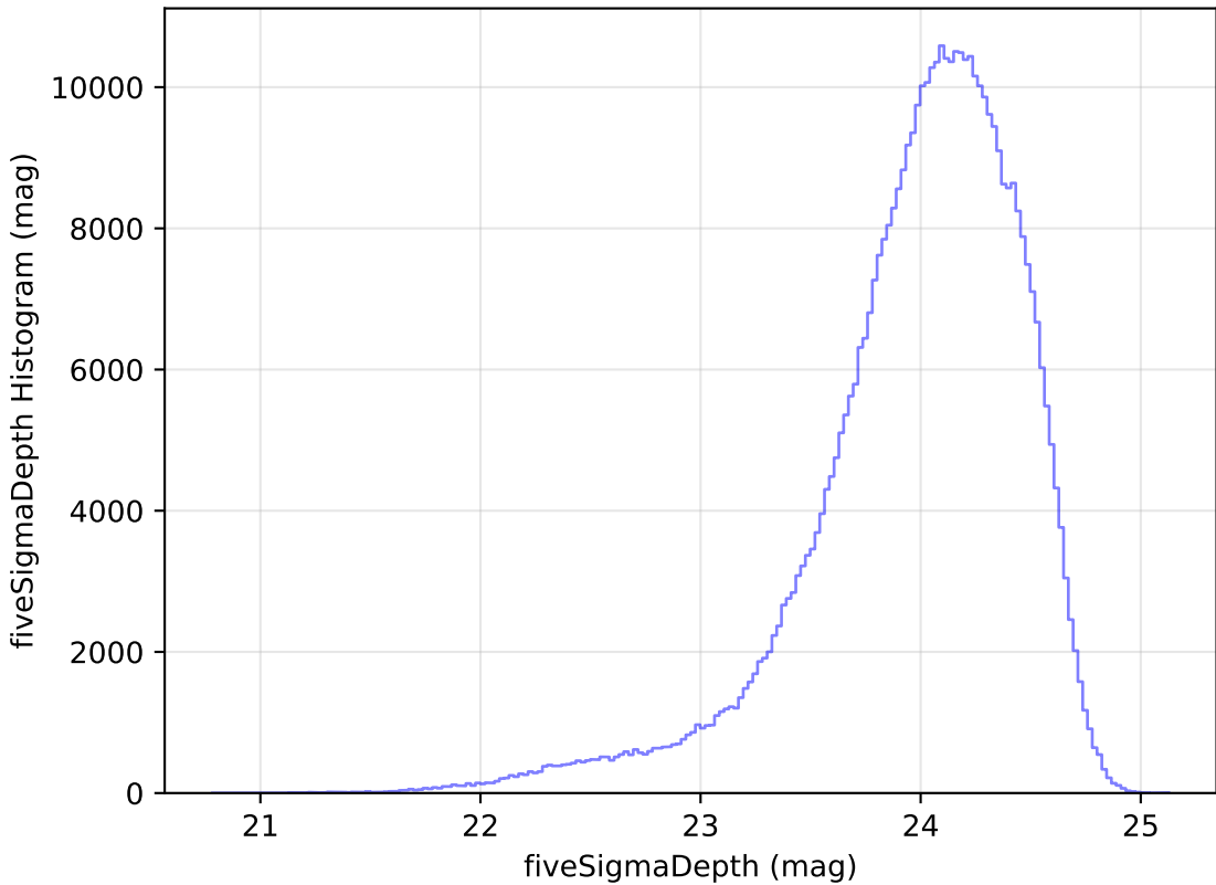
too_5_1v3.4_10yrs All sky r band: fiveSigmaDepth Histogram
