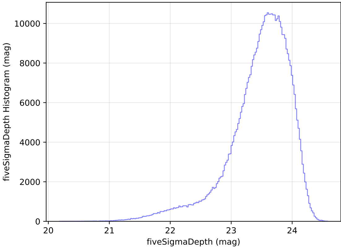
too_5_1v3.4_10yrs All sky i band: fiveSigmaDepth Histogram
