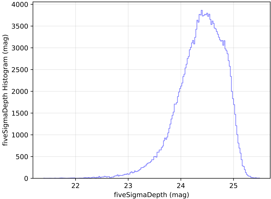
too_5_1v3.4_10yrs All sky g band: fiveSigmaDepth Histogram
