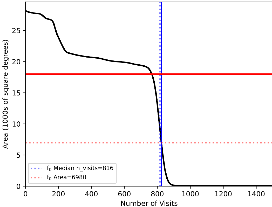
too_5_1v3.4_10yrs All sky: f0
