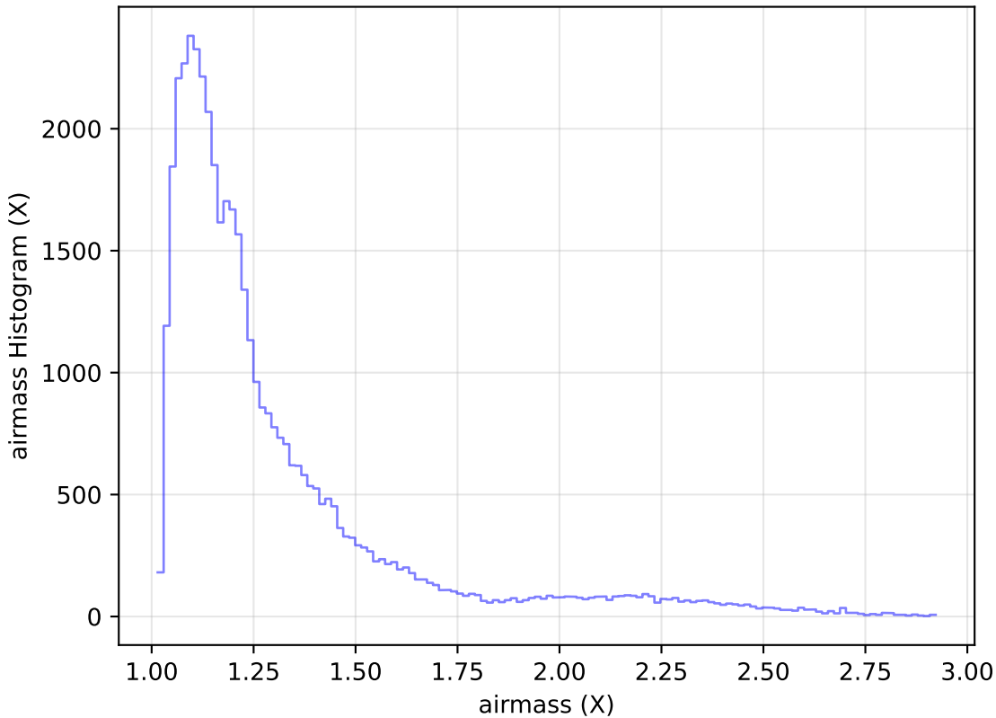
too_5_1v3.4_10yrs Yr 1 z band: airmass Histogram
