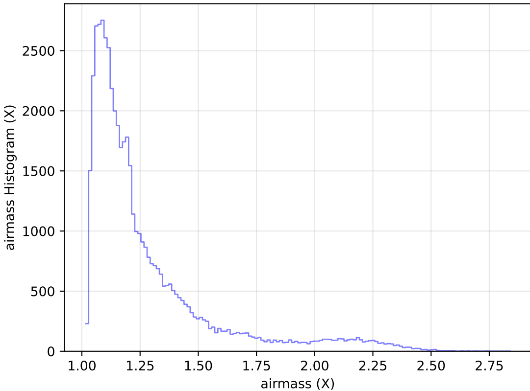
too_5_1v3.4_10yrs Yr 1 r band: airmass Histogram
