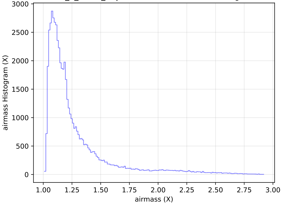
too_5_1v3.4_10yrs Yr 1 i band: airmass Histogram
