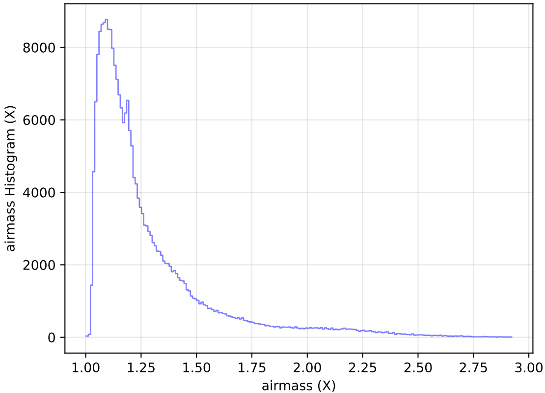
too_5_1v3.4_10yrs Yr 1 all bands: airmass Histogram
