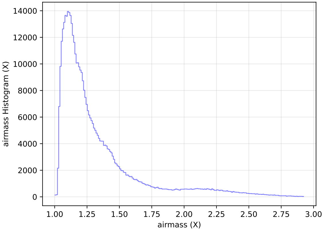
too_5_1v3.4_10yrs WFD z band: airmass Histogram
