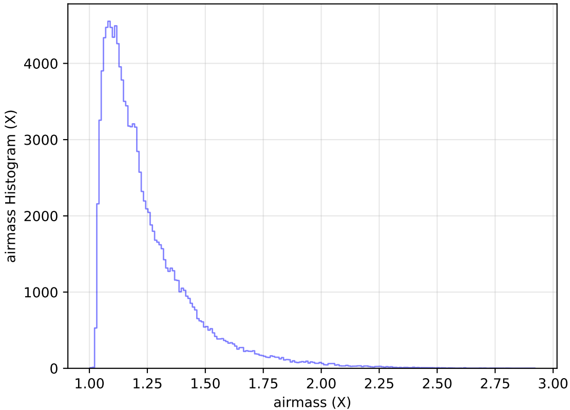
too_5_1v3.4_10yrs WFD u band: airmass Histogram
