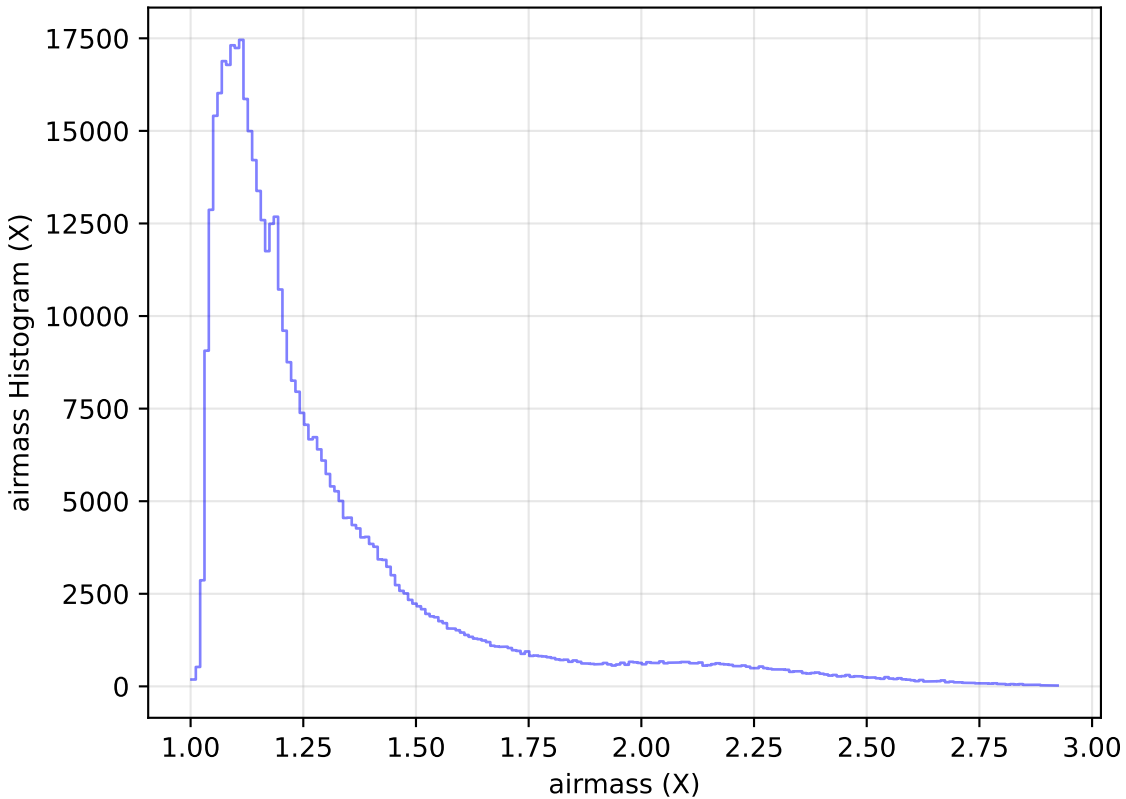
too_5_1v3.4_10yrs WFD i band: airmass Histogram
