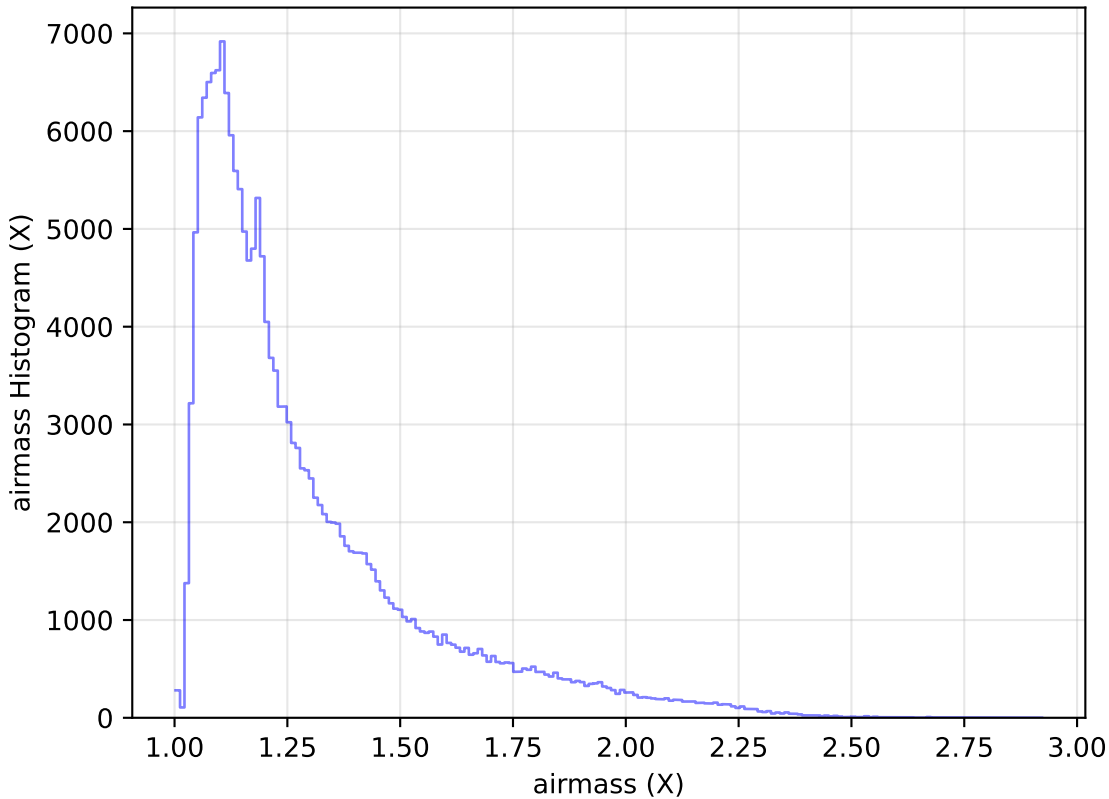
too_5_1v3.4_10yrs WFD g band: airmass Histogram
