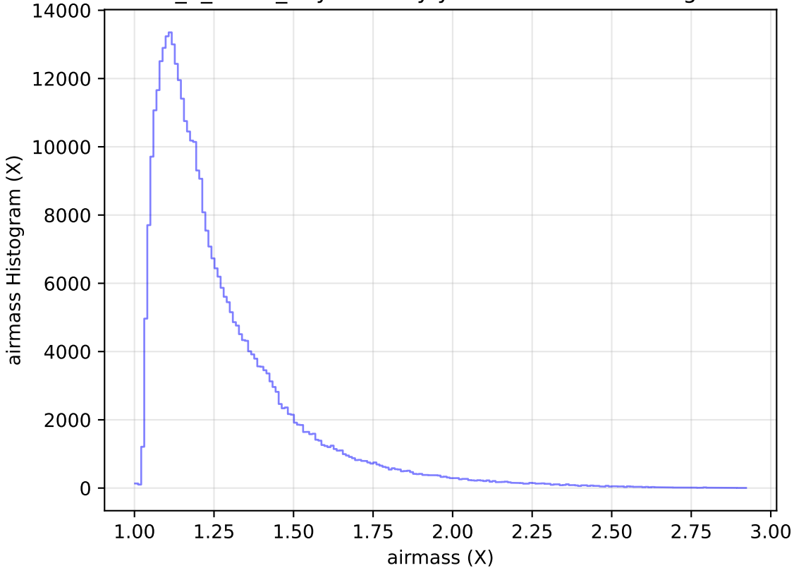
too_5_1v3.4_10yrs All sky y band: airmass Histogram
