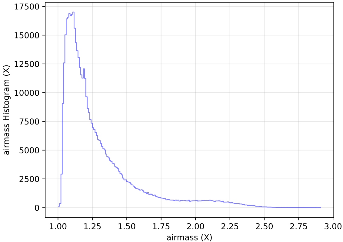
too_5_1v3.4_10yrs All sky r band: airmass Histogram
