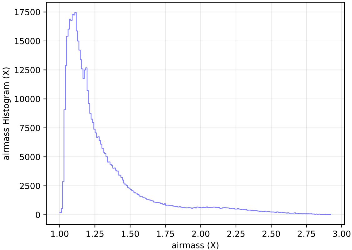
too_5_1v3.4_10yrs All sky i band: airmass Histogram
