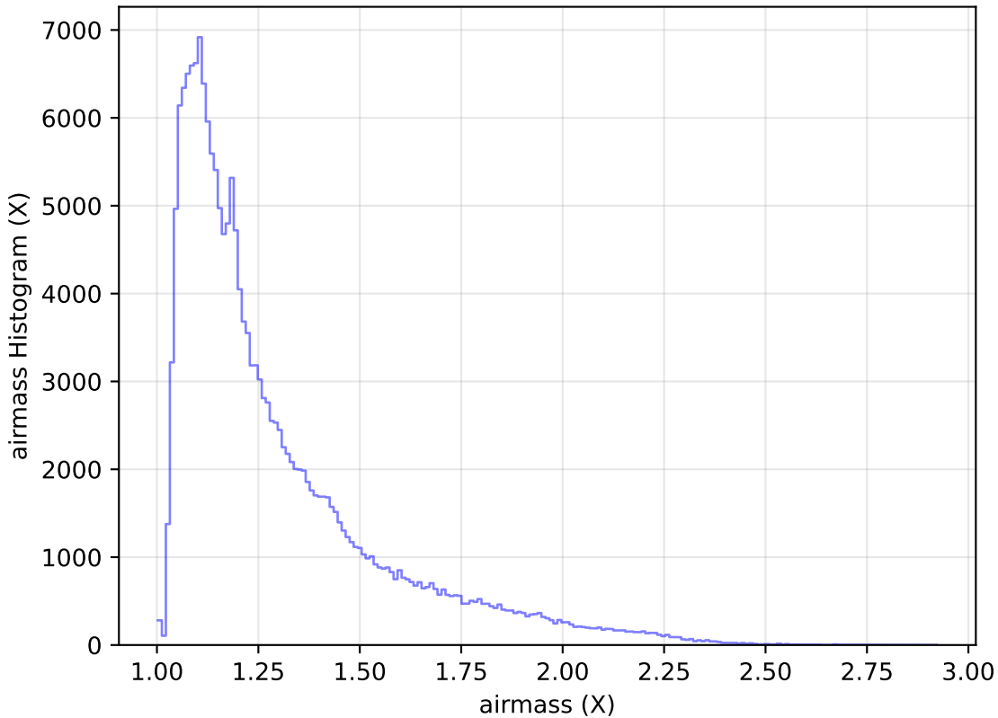
too_5_1v3.4_10yrs All sky g band: airmass Histogram
