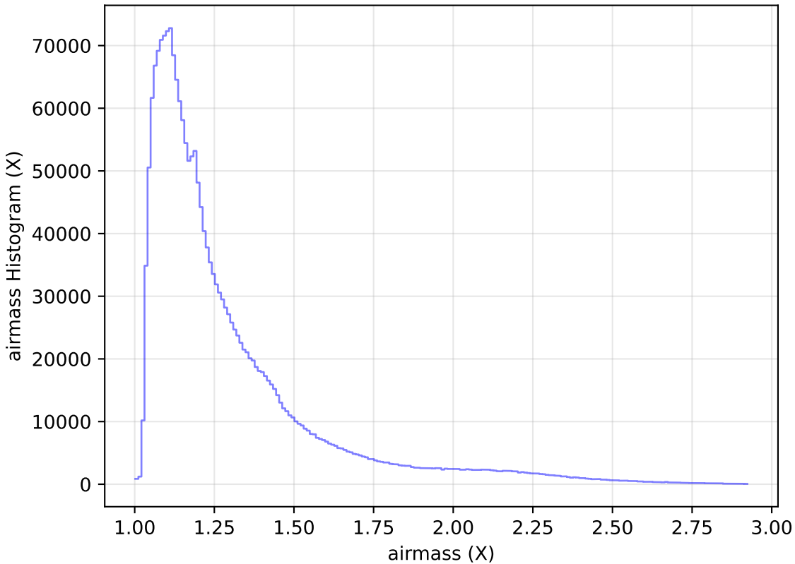
too_5_1v3.4_10yrs All sky all bands: airmass Histogram
