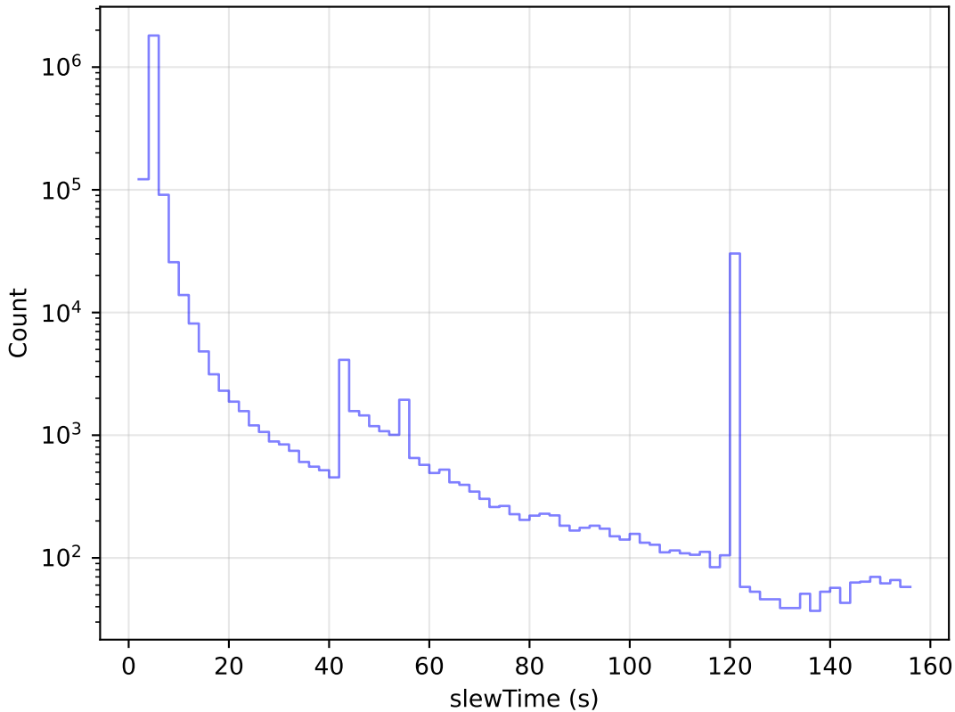
too_5_1v3.4_10yrs All visits: Slew Time Histogram
