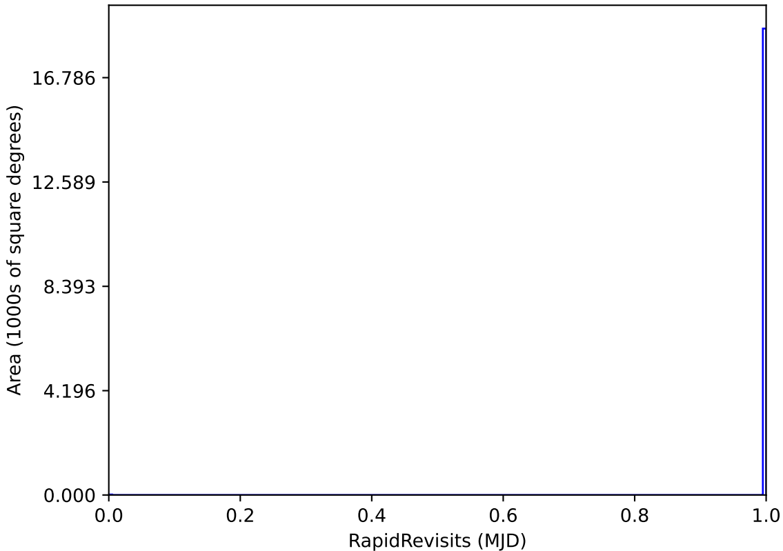
too_5_1v3.4_10yrs WFD: RapidRevisits
