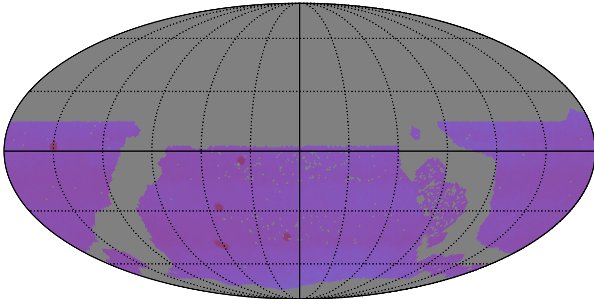
too_5_1v3.4_10yrs WFD: Proper Motion Uncert @ 20.5
