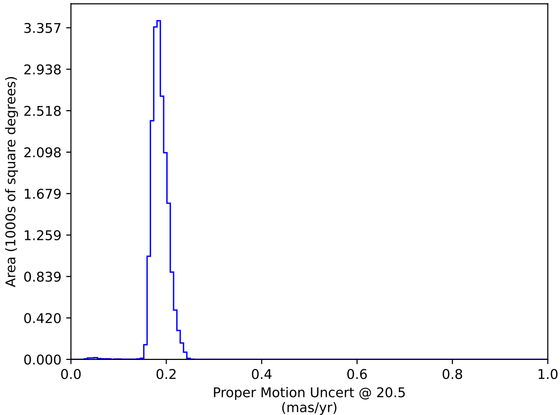
too_5_1v3.4_10yrs WFD: Proper Motion Uncert @ 20.5
