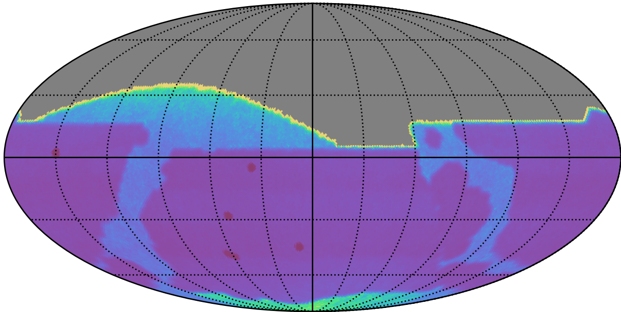
too_5_1v3.4_10yrs All sky: Proper Motion Uncert @ 20.5
