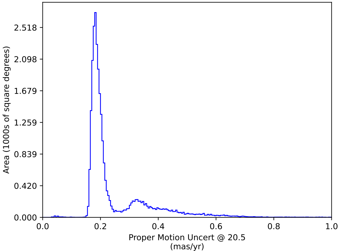
too_5_1v3.4_10yrs All sky: Proper Motion Uncert @ 20.5
