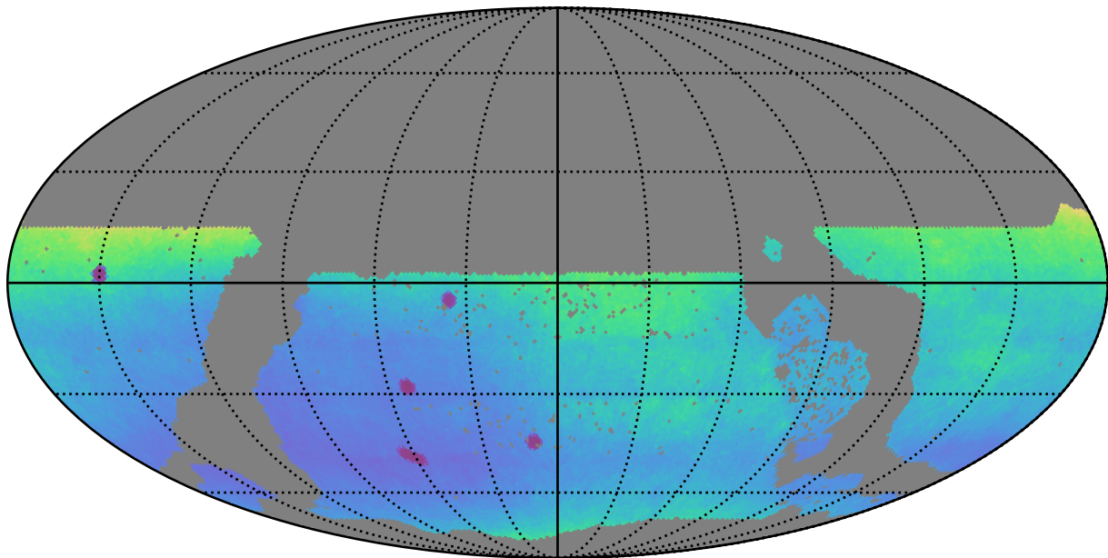
too_5_1v3.4_10yrs WFD: Parallax Uncert @ 24.0
