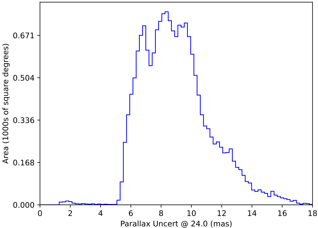
too_5_1v3.4_10yrs WFD: Parallax Uncert @ 24.0
