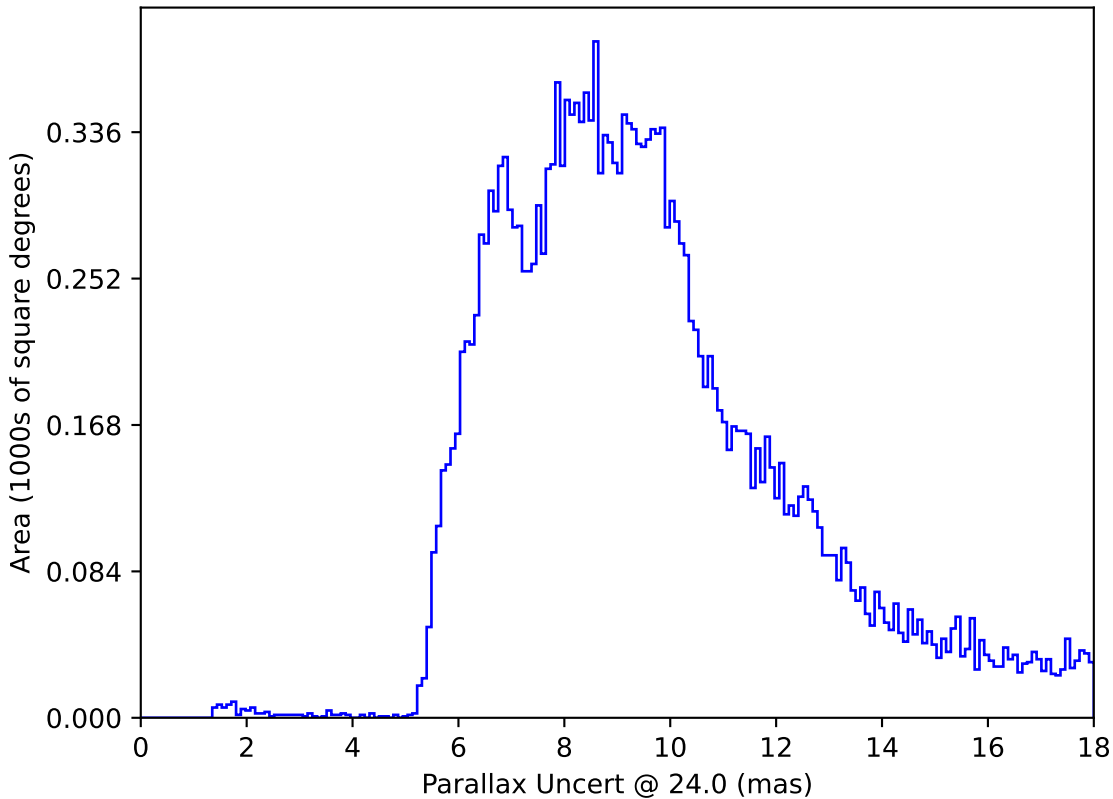
too_5_1v3.4_10yrs All sky: Parallax Uncert @ 24.0
