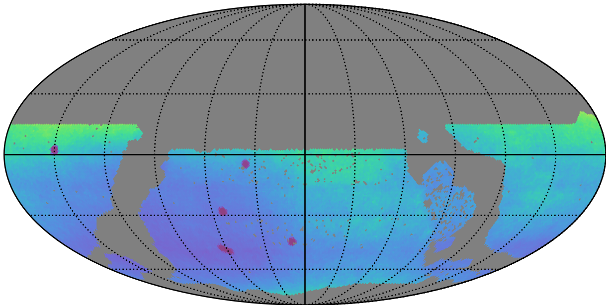
too_5_1v3.4_10yrs WFD: Parallax Uncert @ 22.4
